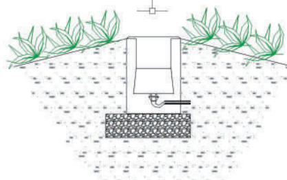
Incorrect Fixing method Do not install on hollow areas
